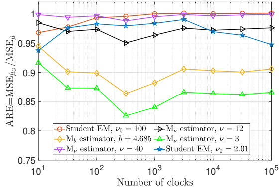
Fig. 1. Asymptotic Relative Efficiency (ARE) for the investigated robust estimators in the absence of anomalies. The closer the ARE to 1, the better the associated estimator performs under nominal conditions.
