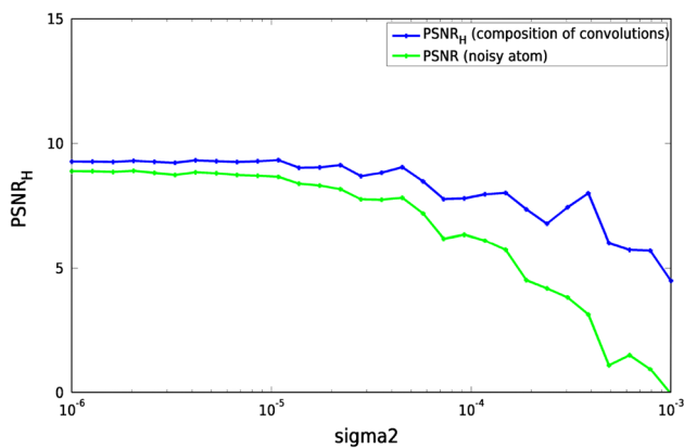
Fig. 4 PSNR_H for the approximation of the apodized frequency 100 MDC by the convolution of K = 9 kernels of sparsity S = 9 , for 10^{-6} \leq \sigma^2 \leq 10^{-3} (blue curve). The green curve is the PSNR between u and \alpha * H (Color figure online)
