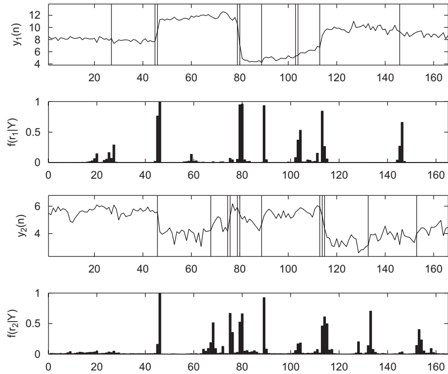
Fig. 10. Posterior distributions of the change-point locations and segmentation of real data obtained after N_{\text{bi}} = 1000 burn-in iterations and N_{\text{r}} = 8000 iterations of interest.
