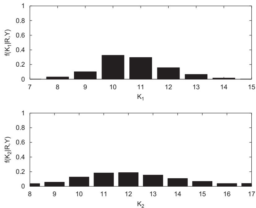
Fig. 11. Posterior distributions of the change-point numbers computed from N_{\text{r}} = 8000 iterations of interest.
