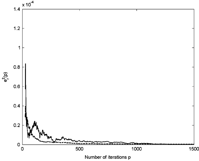
Fig. 5. MSE between the reference and estimated a posteriori change-point probabilities versus p (solid line). Averaged MSE computed from 10 chains (dashed line) ( N_{bi} = 100 ).
