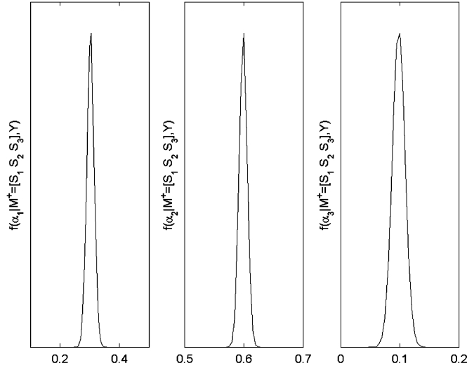
Fig. 13. Posterior distribution of the estimated abundances \alpha^+ = [\alpha_1, \alpha_2, \alpha_3]^T conditioned upon R = 3 and M^+ = [s_1, s_2, s_3] .
