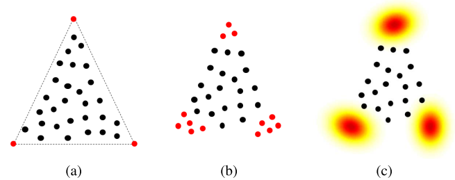
Fig. 1. Simplex representation for (a) endmembers without variability, (b) endmembers as a finite set (or bundle) and (c) endmembers as a distribution.
