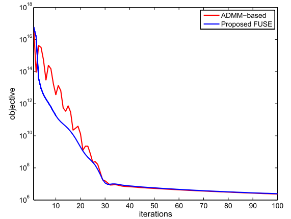
Fig. 3. Convergence speeds of the ADMM [24] and the proposed FUSE-ADMM with the TV-regularization.
